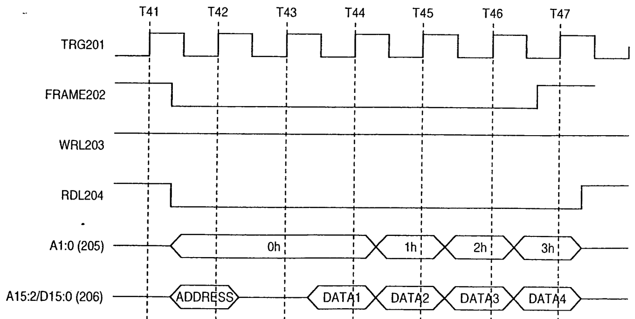
FIG. 19 PRIOR ART
